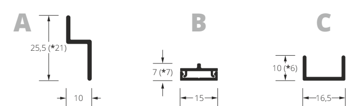
Bottom guide channels.
