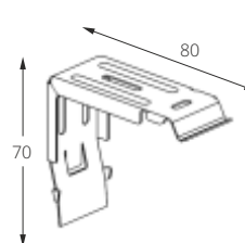
■ bracket.
